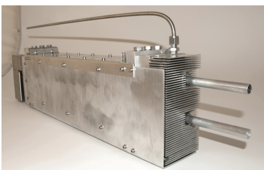
Brintreformer - prototype
